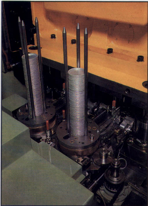
SHELL FEEDING
